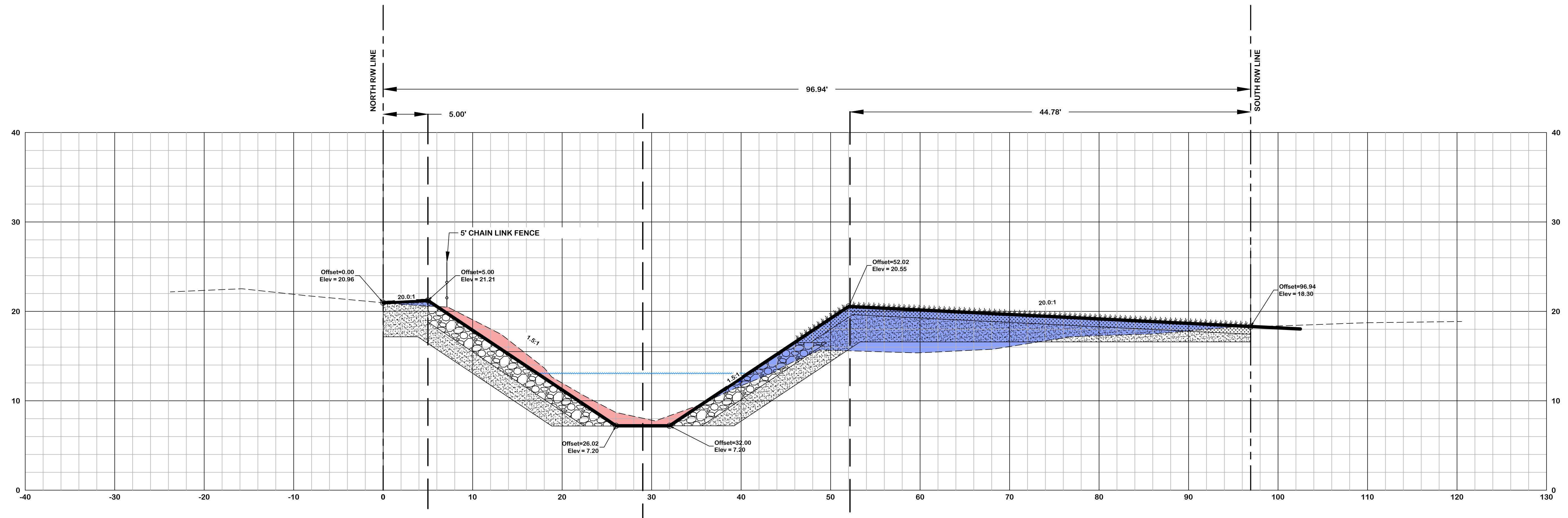
EXISTING CANAL CROSS SECTION #3 CROSS SECTION LOOKING EAST SCALE: 1" = 10' (H&V)
