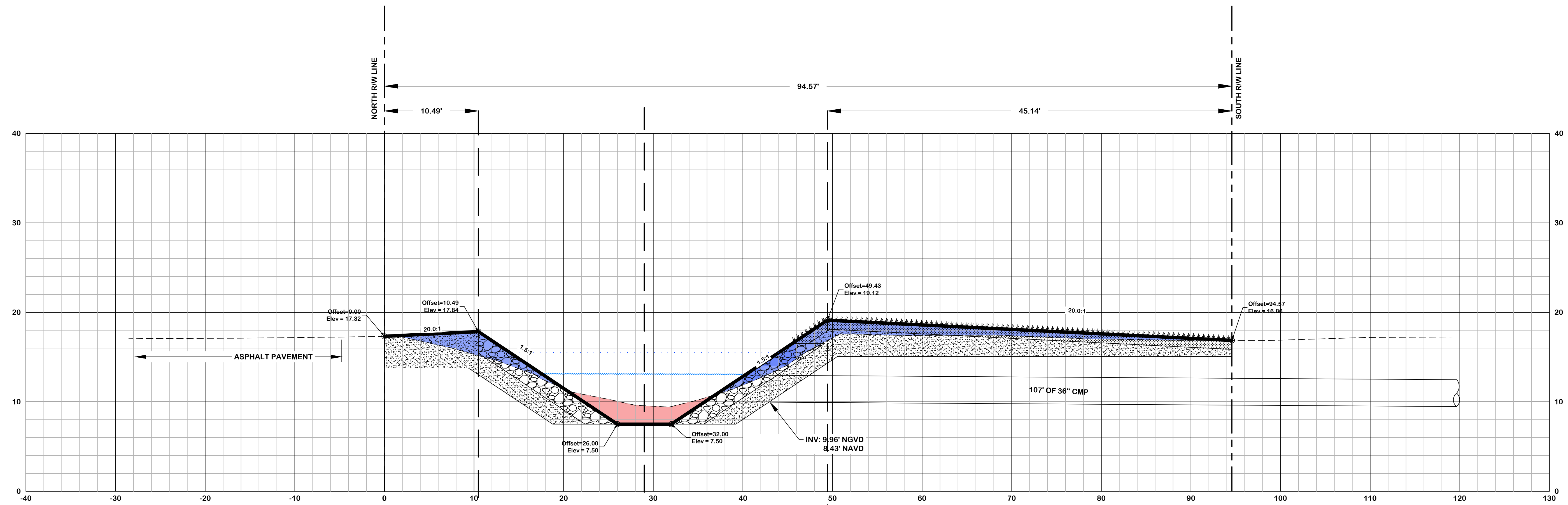
EXISTING CANAL CROSS SECTION #1 CROSS SECTION LOOKING EAST SCALE: 1" = 10' (H&V)
