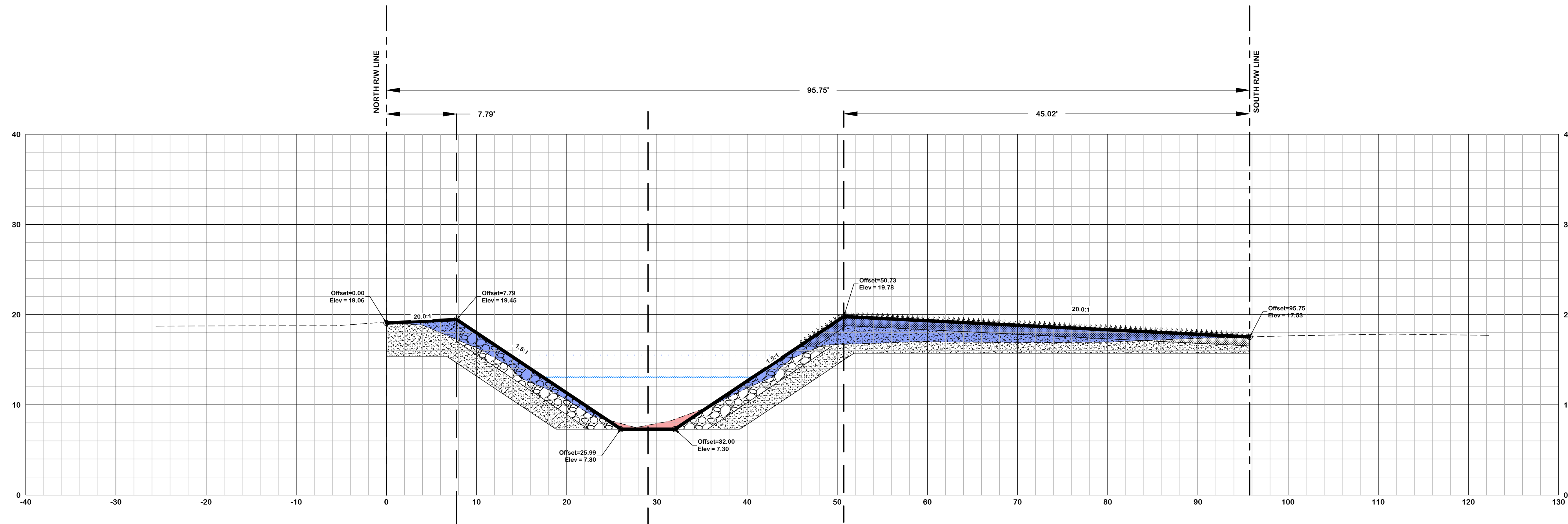
EXISTING CANAL CROSS SECTION #2 CROSS SECTION LOOKING EAST SCALE: 1" = 10' (H&V)
