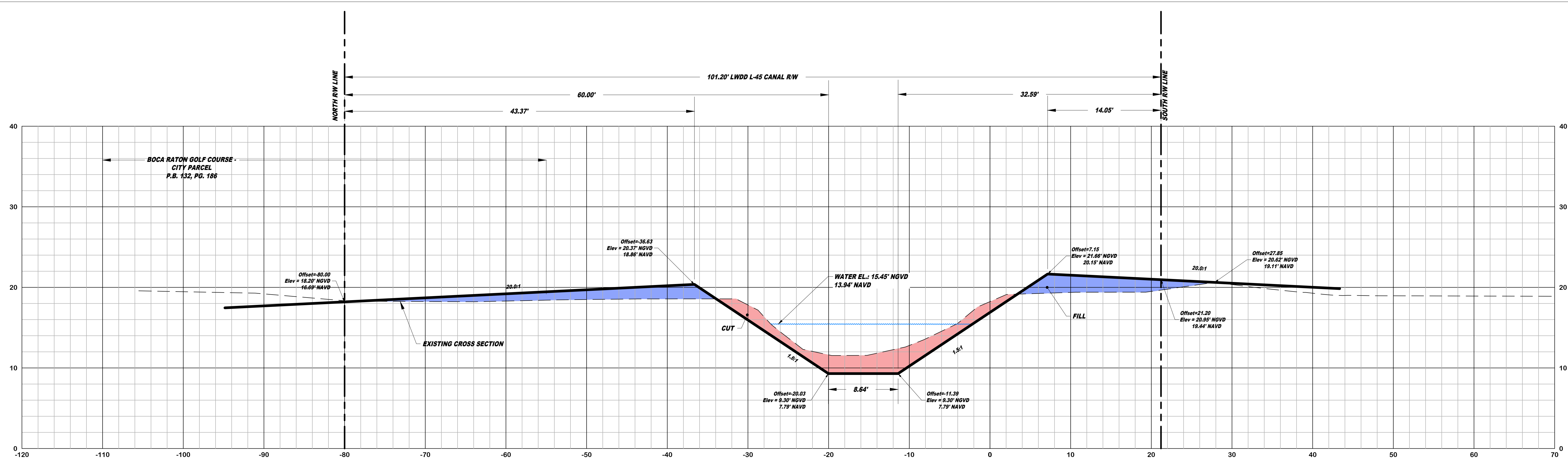
EXISTING CANAL CROSS SECTION #18 CROSS SECTION LOOKING EAST SCALE: 1" = 10' (H&V)
