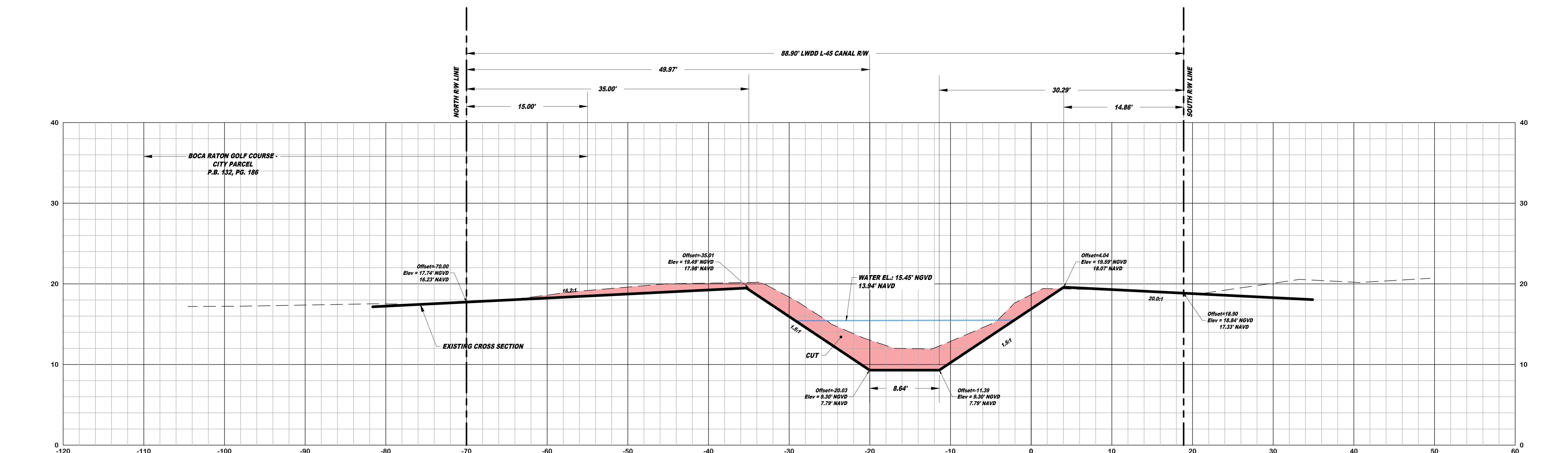
EXISTING CANAL CROSS SECTION #19 CROSS SECTION LOOKING EAST SCALE: 1" = 10' (H&V)
